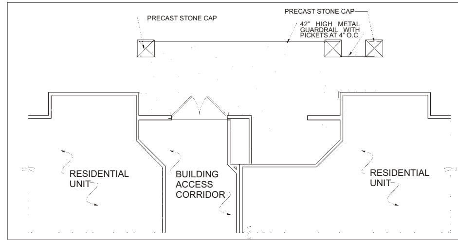
PRIVATE STOOP PLAN DETAIL BUILDING ACCESS CORRIDOR
