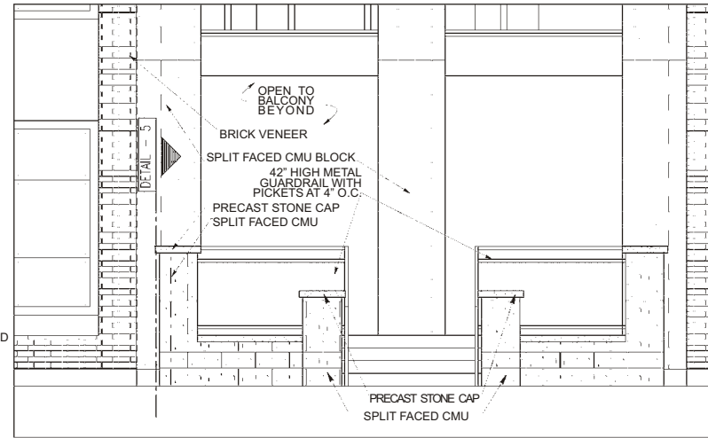
TYP. FRONT DETAIL OF STOOP
