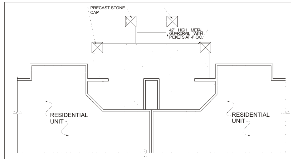
TYPICAL PRIVATE STOOP PLAN DETAIL
